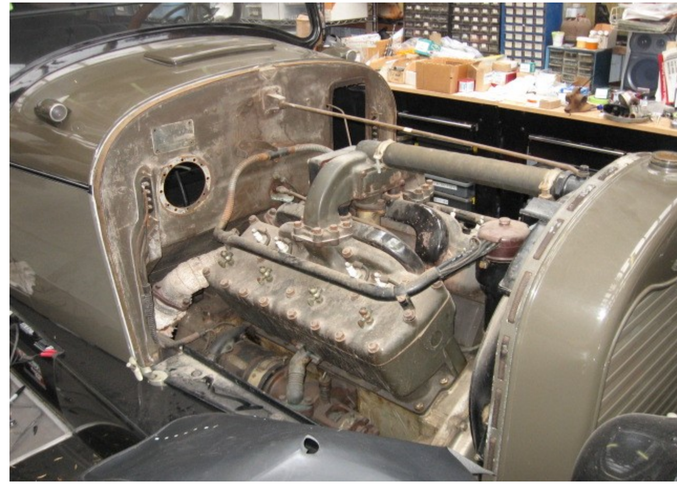
Arrival Photo - not run in 32 years
