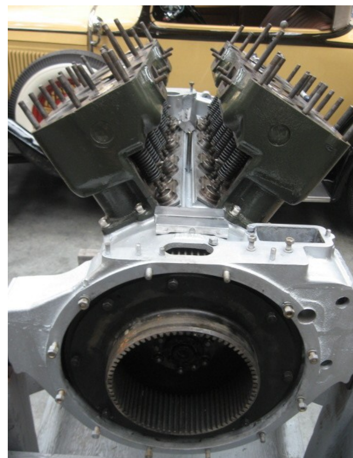
Cylinders, Flywheel mounted
