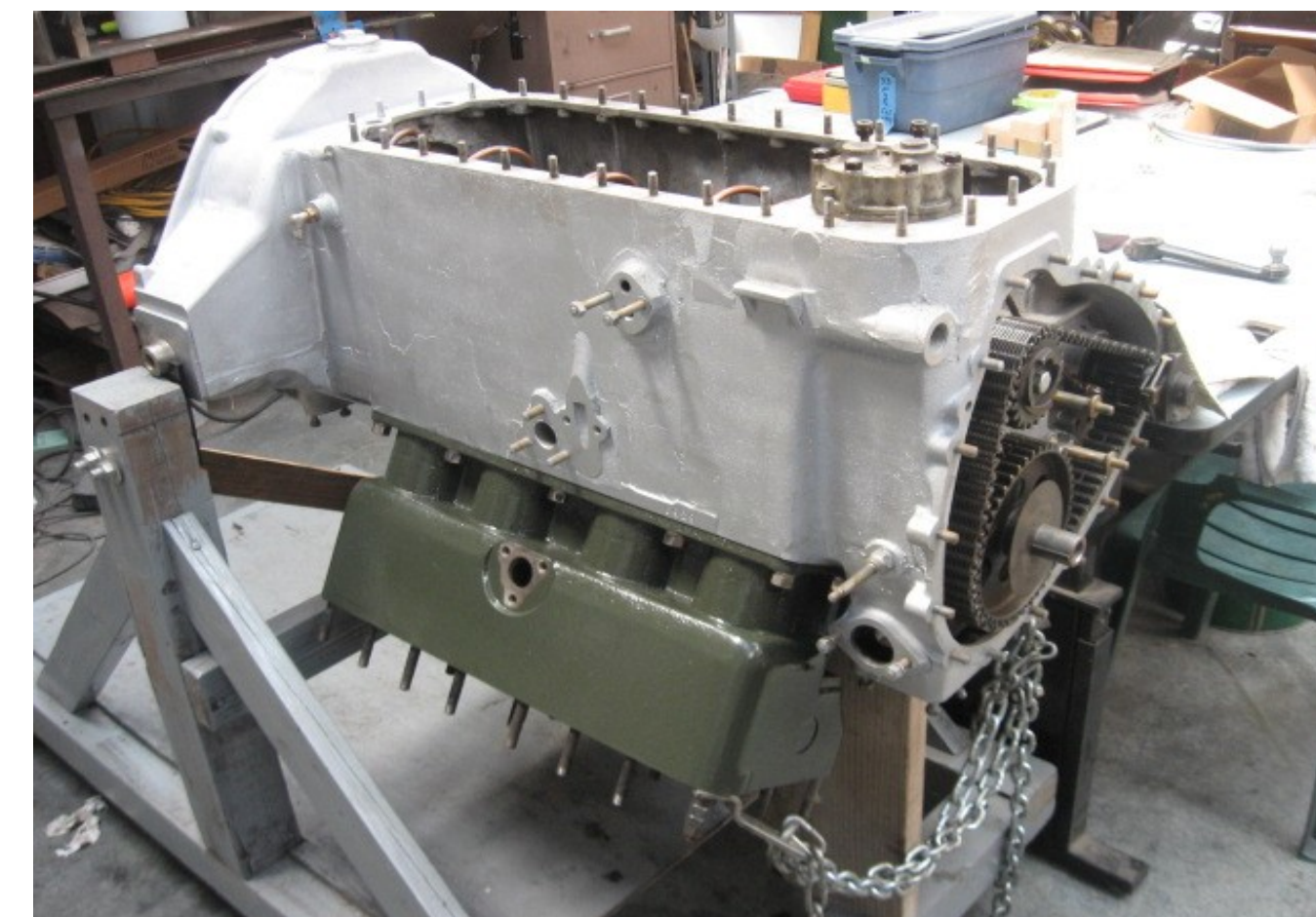
Check timing on cam
